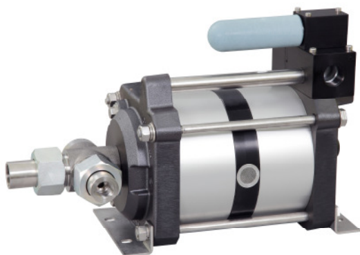
G100-2 (L) single acting, double air drive head (Standard= Bottom inlet)
