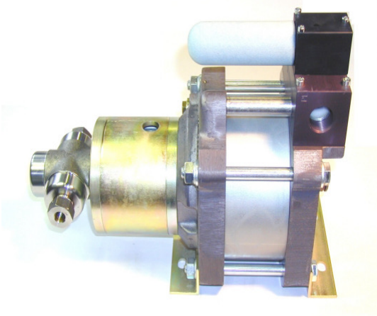
G500 (L)S single acting, single air drive head, side inlet (Bottom inlet not available)
