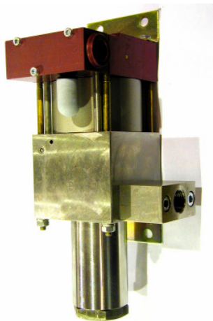
MSF8(L) single acting, single air drive head and distance piece (Standard= Bottom inlet)
